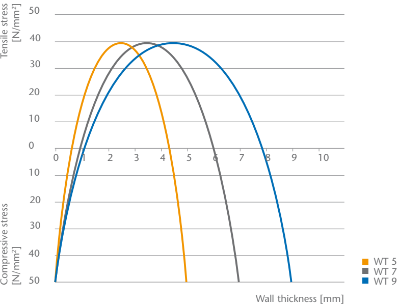
Resulting stress profile in the tubing wall, for various wall thicknesses, such as the tube diameter 120 mm.
